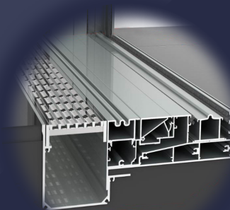
EVOLUTION THRESHOLD DRAIN (optional)
